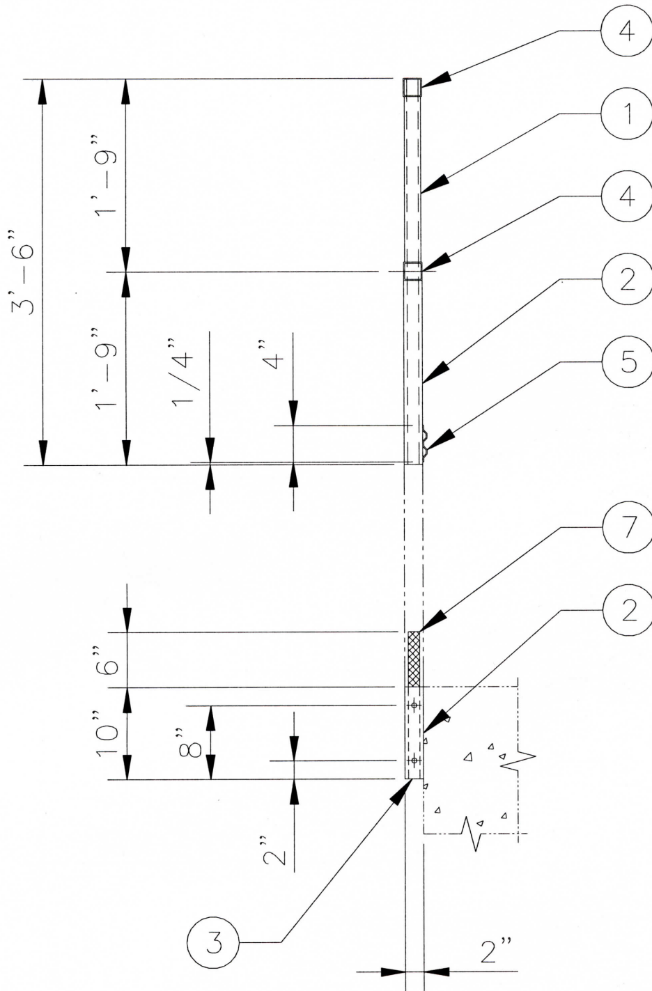
TYP. REMOVABLE FRP HANDRAIL DETAIL
